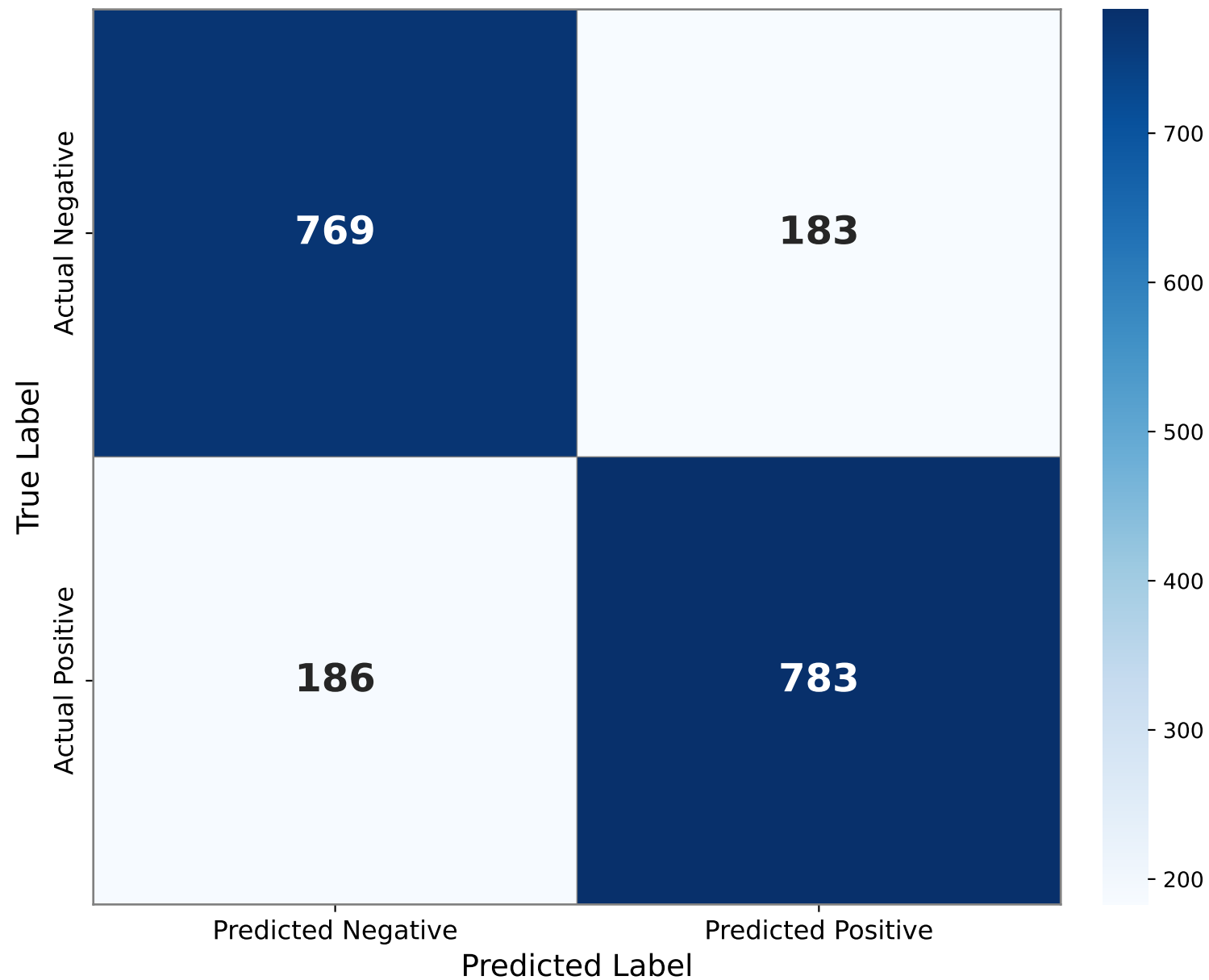
DistilBERT-multilingual-cased
